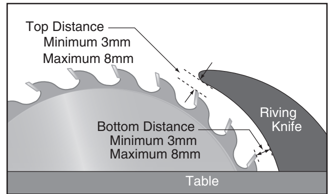
Figure 40. Allowable top and bottom distances between riving knife and blade.
